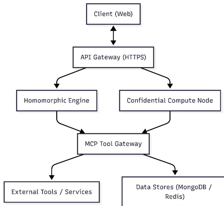
Figure 1 context Diagram
