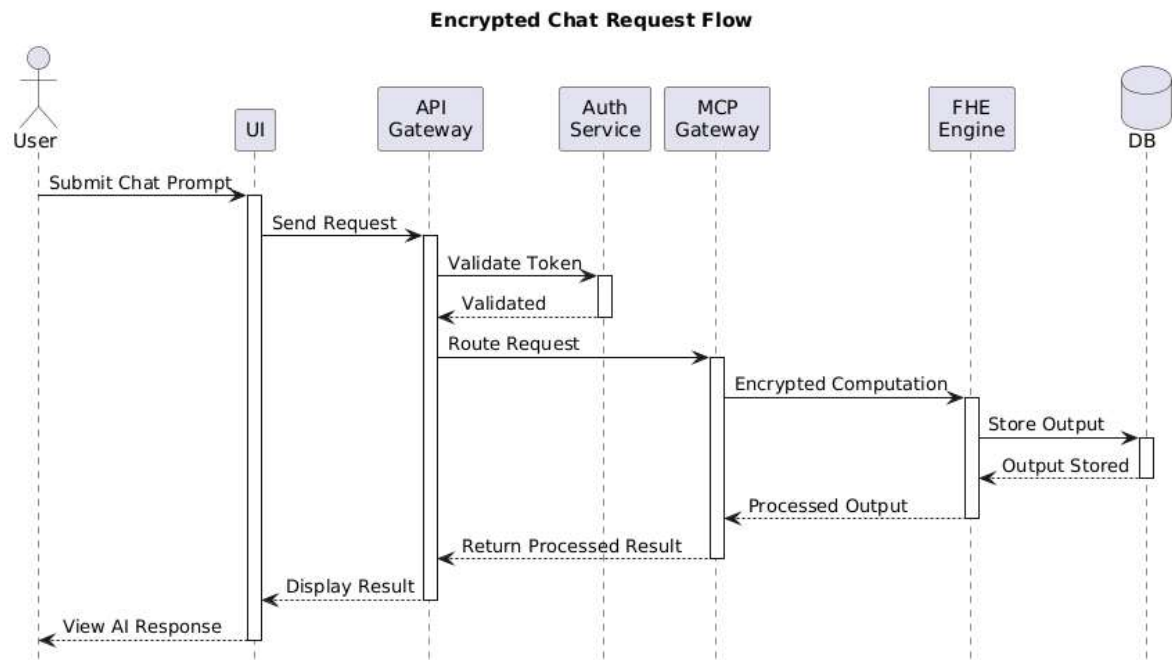
Figure 4 Sequence Diagram
